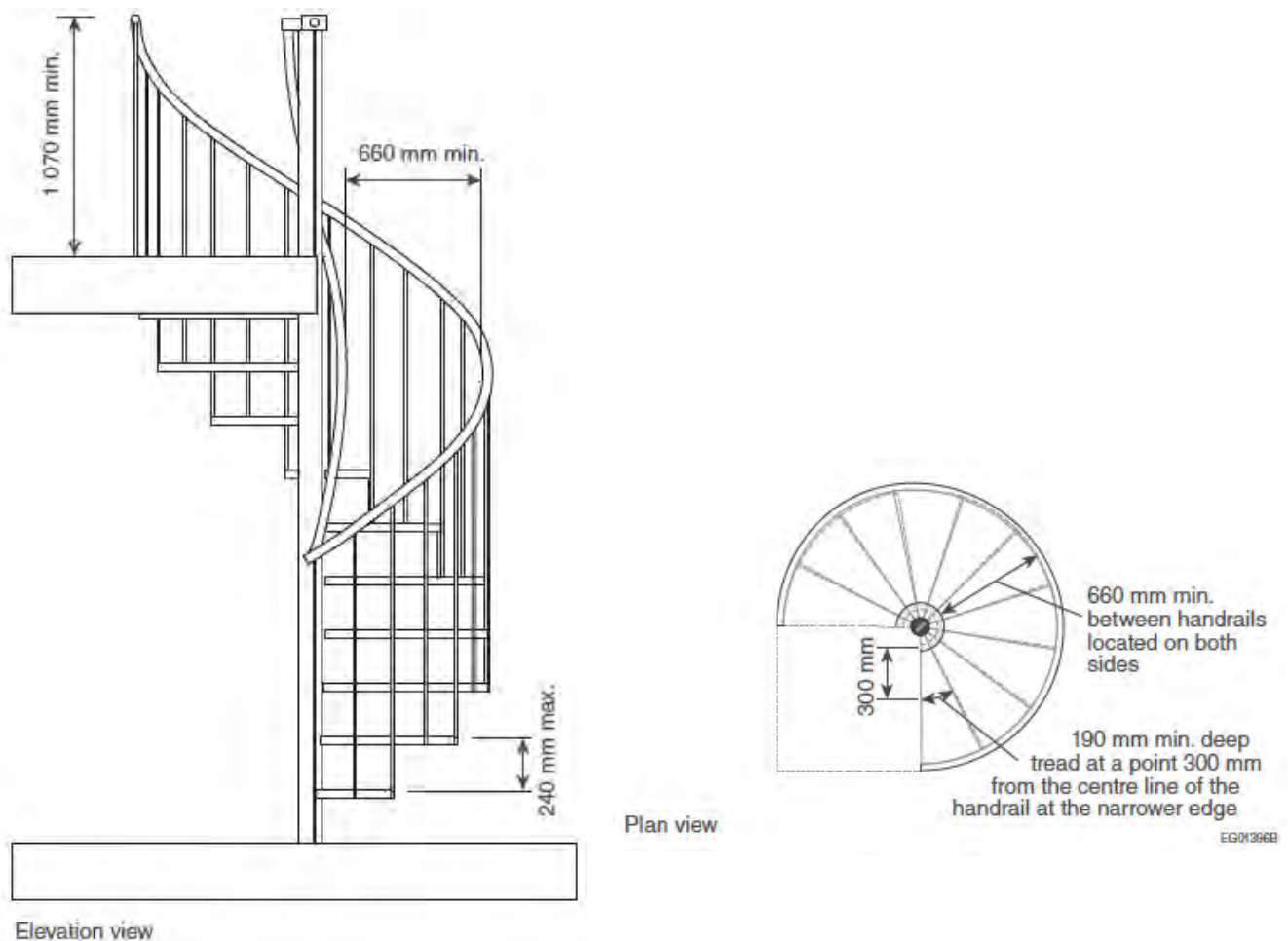
Figure A-9.8.4.7. Spiral Stairs
