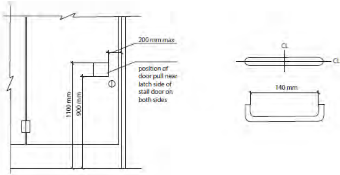
Door Pull Location
