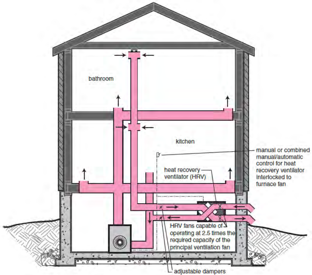
Figure A-9.32.3.3.-F Ventilation System Coupled With a Forced Air Heating System and Using a Heat Recovery Ventilator as the Principal Ventilation Fan to Eliminate the Need for Supplemental Fans
