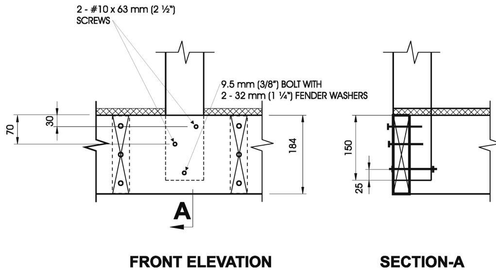
Detail IB-1
