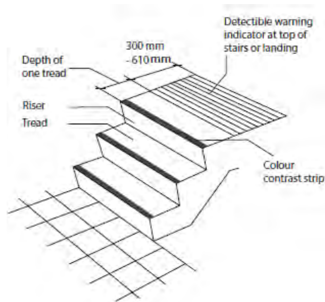
Figure A-3.4.6.1.(1.1) Tactile Indicator at Stairs and Ramps
