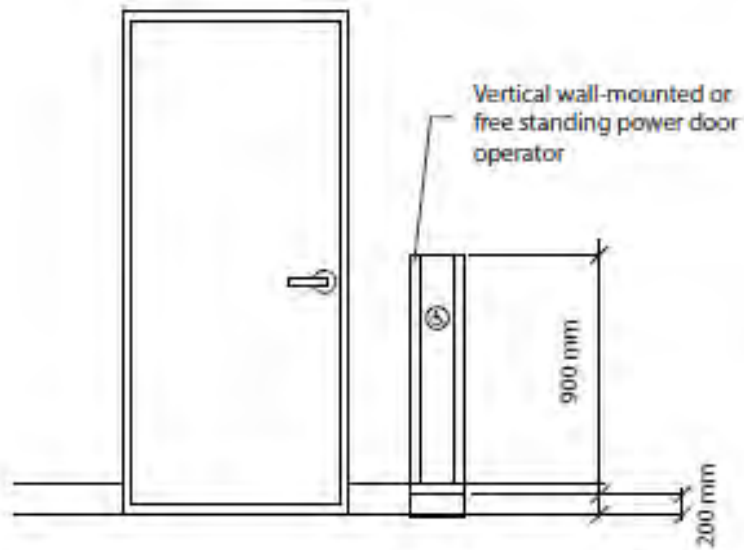
Figure A-3.8.3.3.(17)(c) Vertical Power Door Operator
