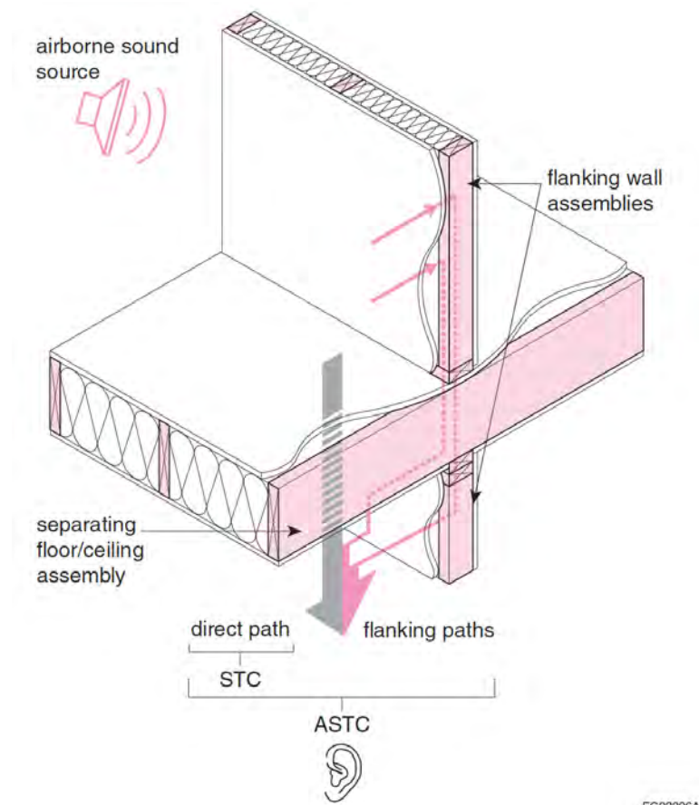
Figure A-9.11.-B Vertical Sound Transmission Paths Floor/Wall Junction
