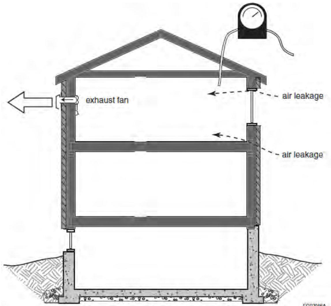
Figure A-9.32.3.8.-B Outdoor Air Drawn Through a Tighter Envelope
