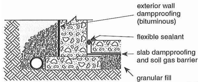
Figure A-9.25.3.3.(9) Dampproofing and Soil Gas Control at Foundation Wall / Floor Junctions with Solid Walls
