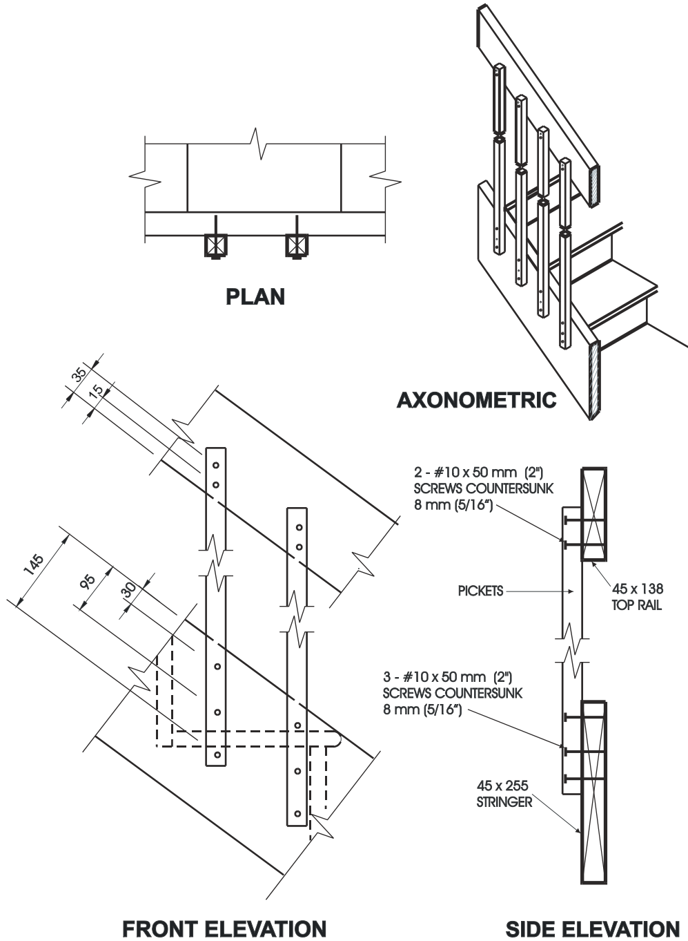
Detail IH-1
