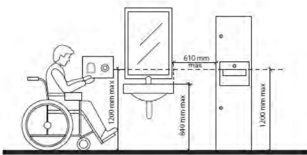
Figure A-3.8.3.11. Washroom Accessories
