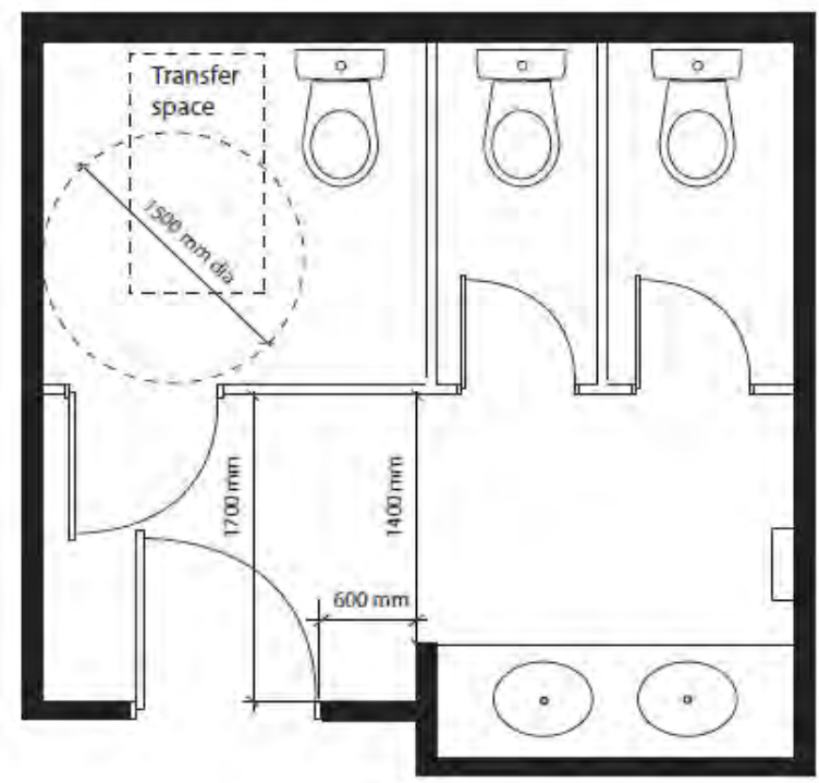
Figure A-3.8.3.8.(1)(f) Washroom Clearances
