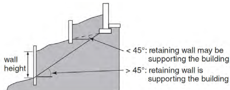
Figure A-9.3.2.9.(4) Identifying Retaining Walls that Require Preservative Treatment
